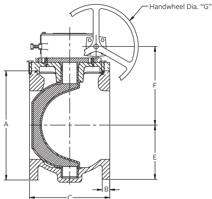
2-1/2" – 12" VALVES
