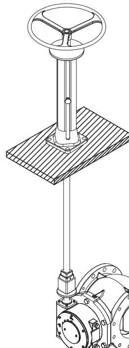
VALVE WITH INDICATING FLOORSTAND
