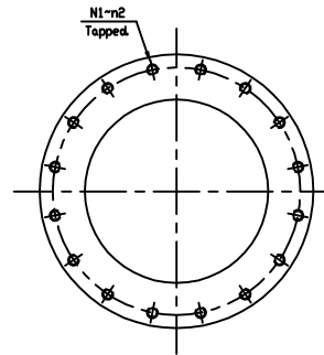
Detail of flange for size 18\"/>
