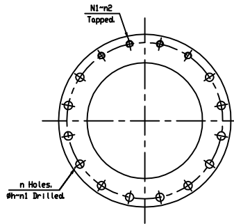
Detail of flange for size 16\"/>
