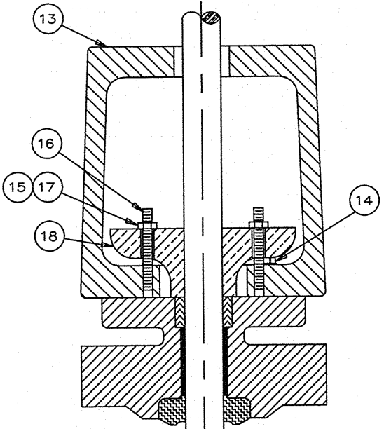
OPTIONAL REPLACEABLE PACKING AND BONNET ASSEMBLY
