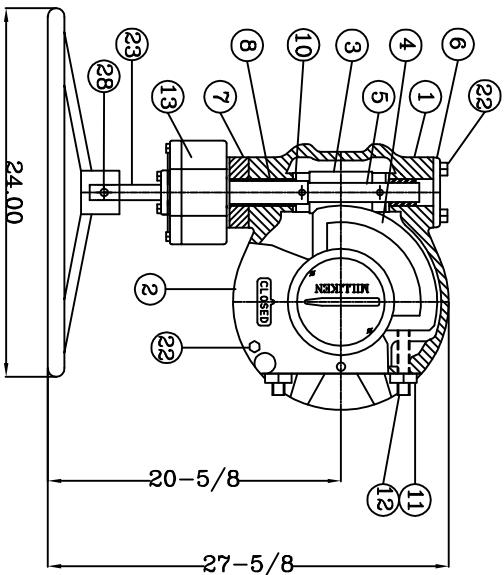
ABOVE GROUND GEAR w/HANDWHEEL
