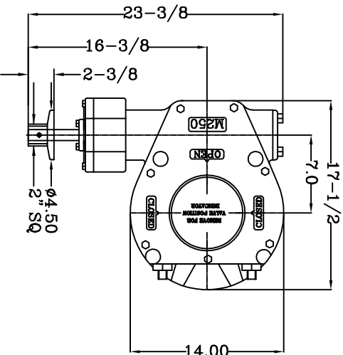
BURIED SERVICE GEAR w/2" NUT
