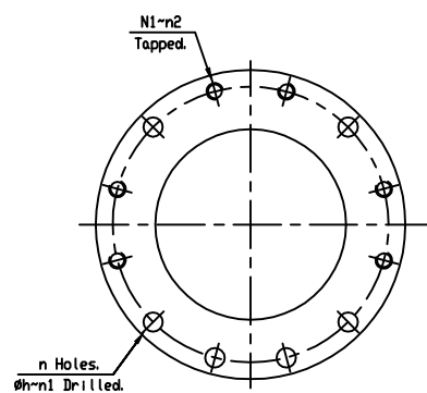
Detail of flange for size 10' (250) only.
