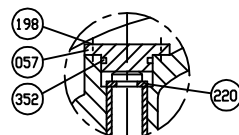
Detail End Plate B
