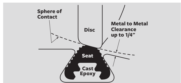
Simple seat adjustment of E-LOK®.
