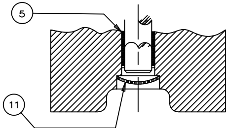
6" THRU 8" VALVES
