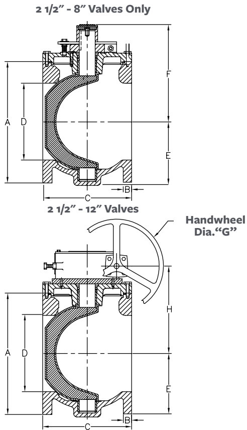
FLANGED END FIG. 2.5" & 3" 601A 4" - 12" 601 175 PSI
