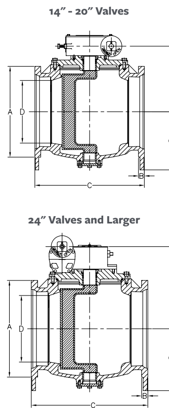
MECHANICAL JOINT END FIG. 600F 150 PSI
