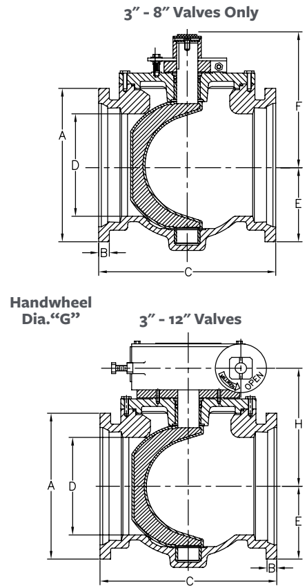
MECHANICAL JOINT END
