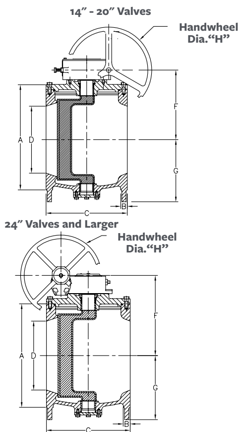
FLANGED END – ANSI 125
