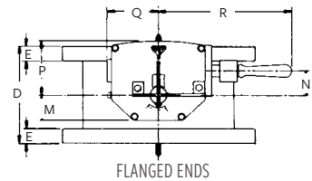
FLANGED ENDS
