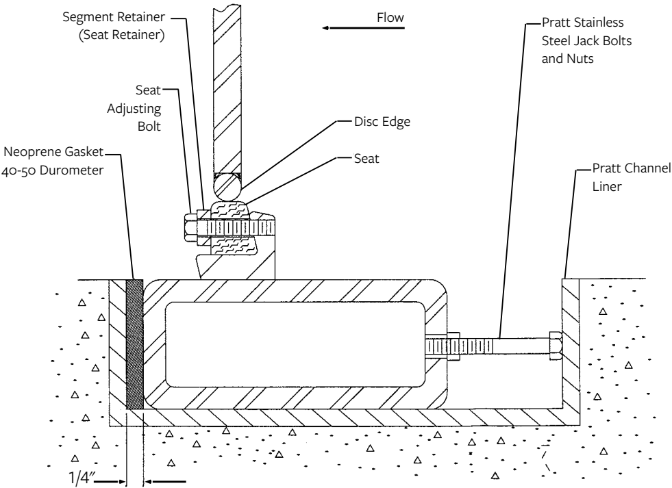
JACK BOLT INSTALLATION DETAIL
