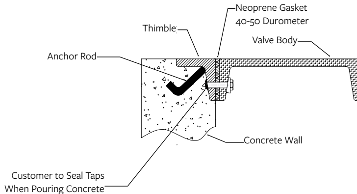
Typical Rectangular Valve with single flange thimble installation.
