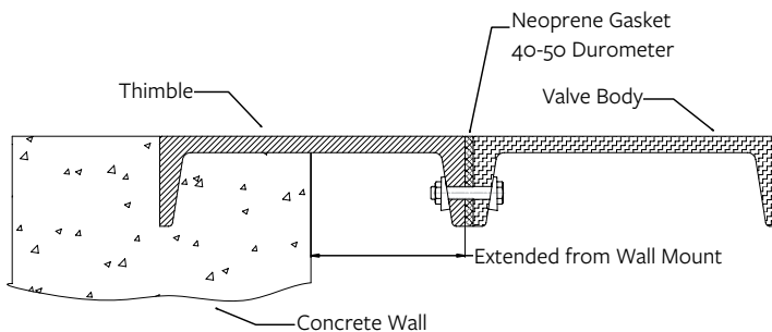
Typical Rectangular Valve with "C" (double flange) thimble installation.
