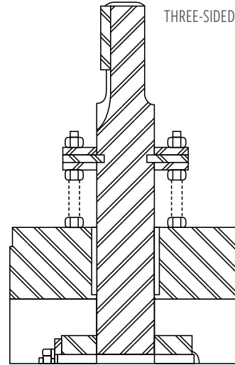
Tight Seal on 3 Sides
