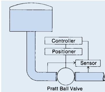
A. PRATT® SET POINT CONTROL SYSTEM
