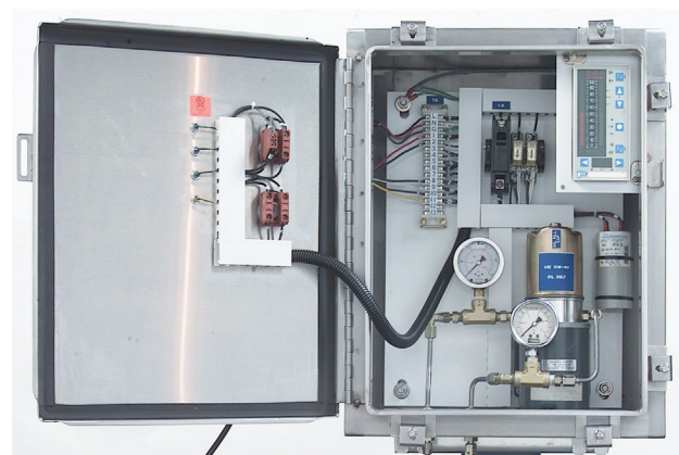
TYPICAL FLOW OR PRESSURE CONTROL SYSTEM
