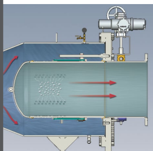
Model 711 Cross Section
