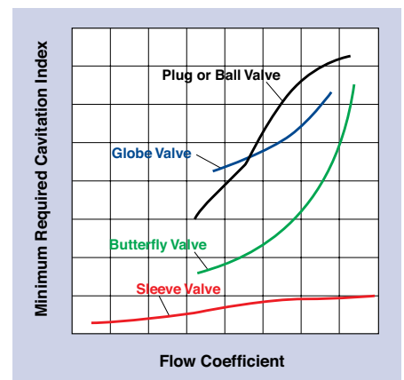
CAVITATION INDEX CURVE
